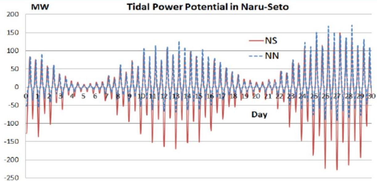
Fig. 19 Variation of tidal power potential calculated at NS and NN sections in Naru-Seto, positive power denotes Northward current and Negative power denotes Southward current
