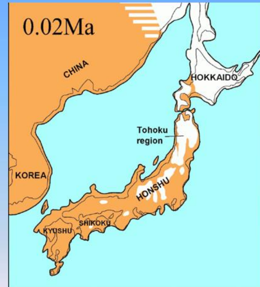
Last Glacial Maximum about 20,000 years ago, thin black line indicates present-day shorelines.
